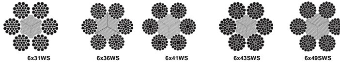
6x36 Class Fiber Core Strength & Weights Chart (inches)
